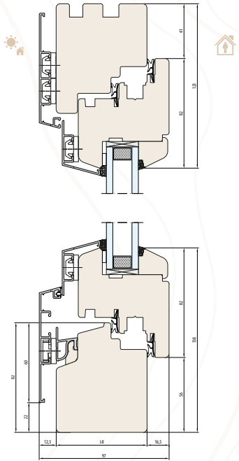
SYSTEM NATURO 68 ALU RENO LINE Without undercut for the window sill
