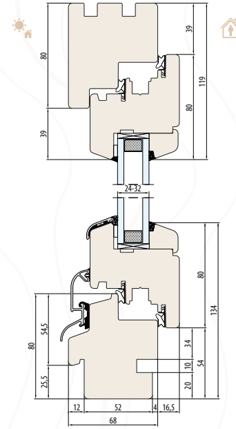
NATURO 68 SYSTEM The undercut for the interior and exterior window sill
