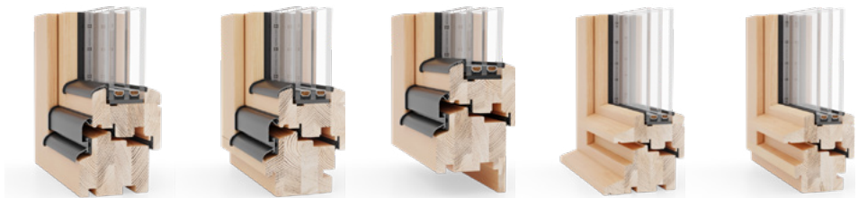
Standard profile (without an undercut)
